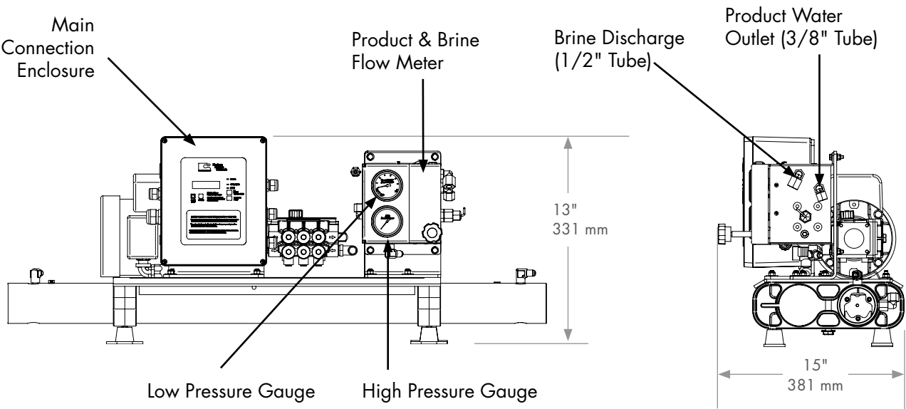
Front View
