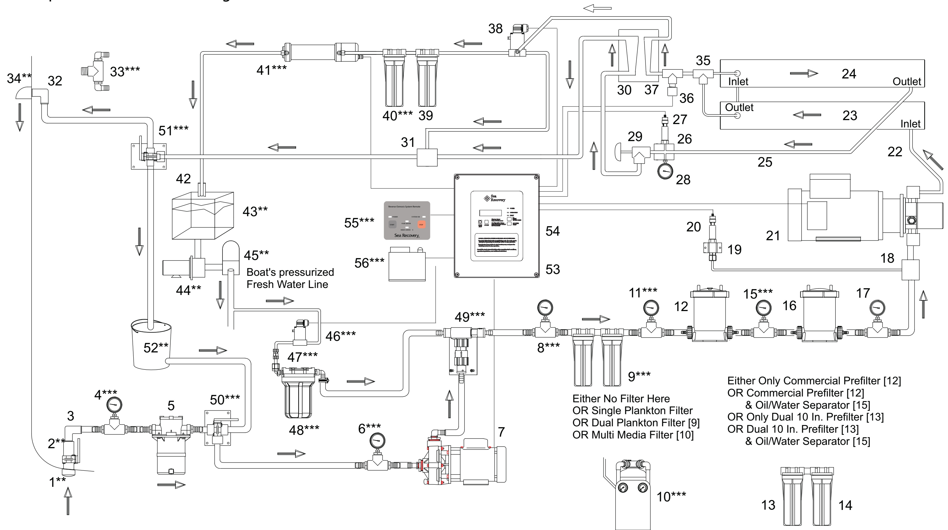
Component Identification Diagram
